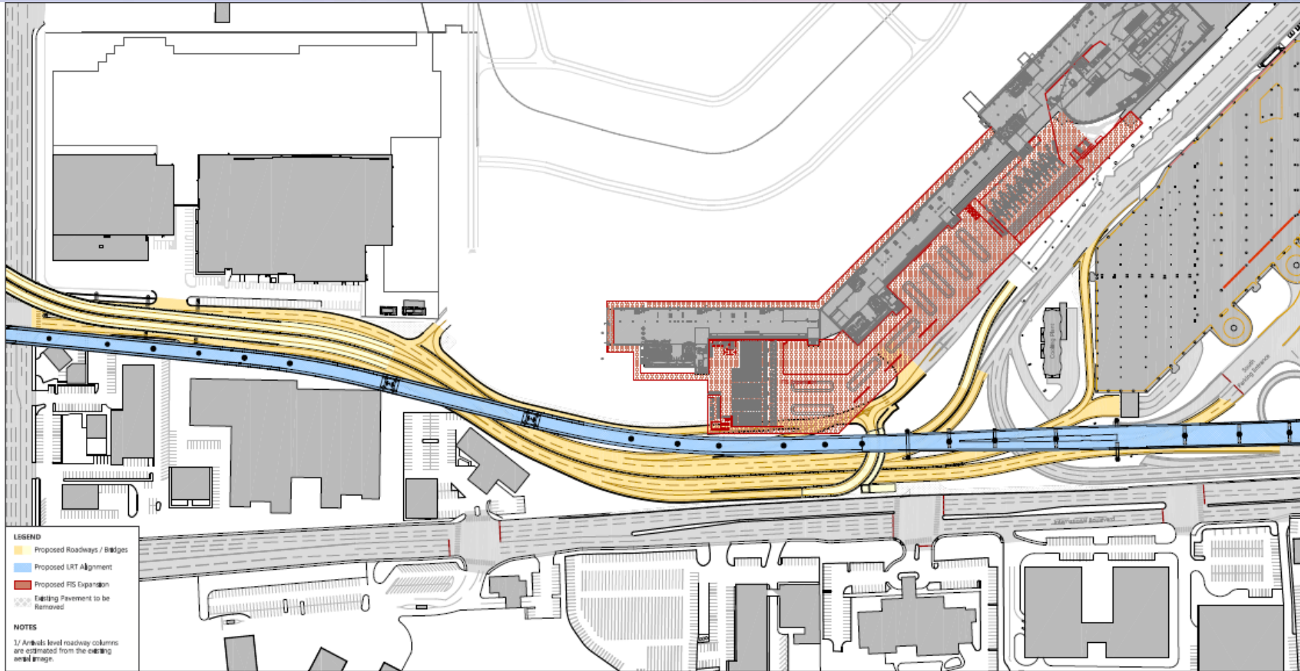
LRT Extension and South Access Roadway - Original Airport Concept South Roadway Modifications - Concept G
